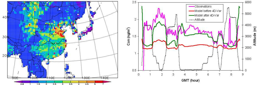
Fig. 14. A-basic methodology of top-down estimates of emissions.
