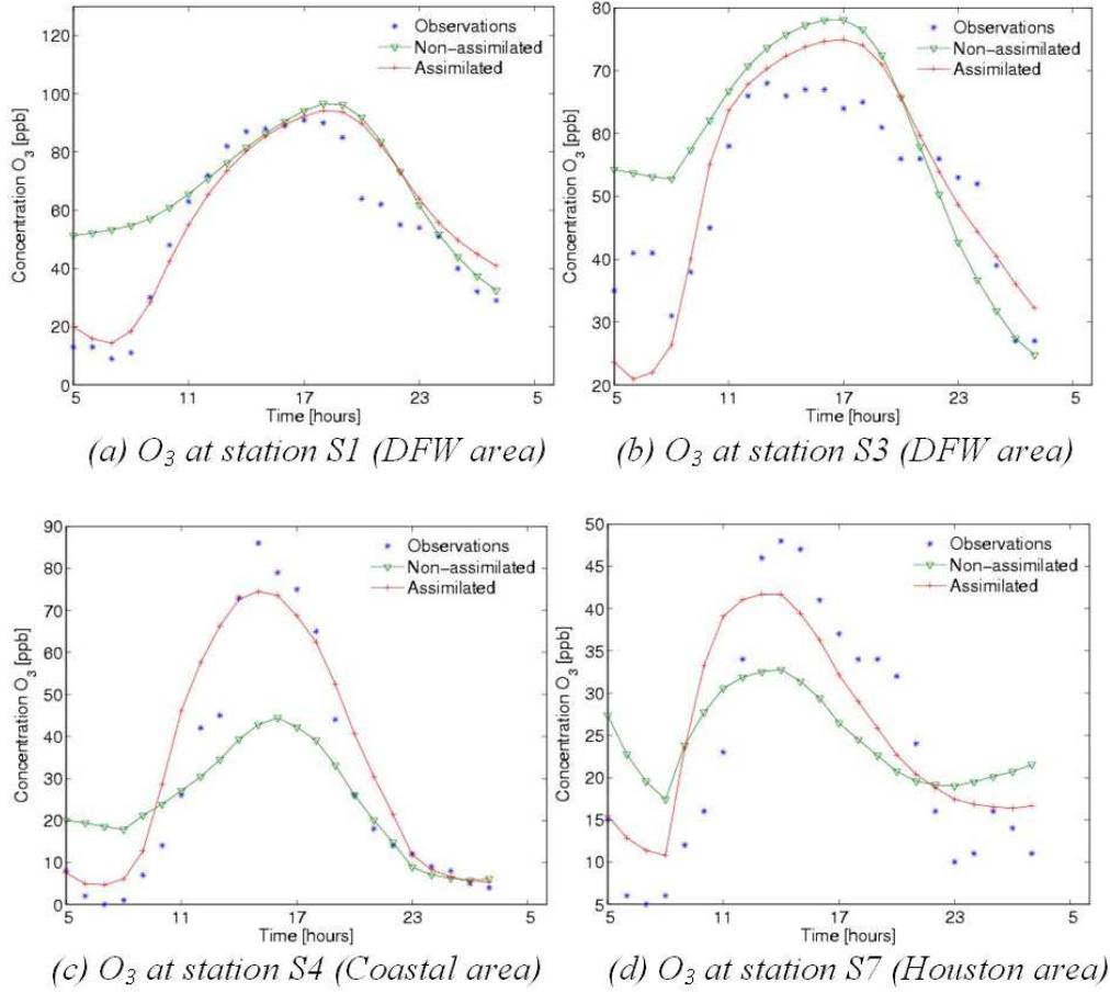
Fig. 11. (a) O_3 at station S1 (DFW area); (b) O_3 at station S3 (DFW area); (c) O_3 at station S4 (Coastal area); (d) O_3 at station S7 (Houston area). Time series of ozone concentrations on July 16, 2004. The concentrations are plotted against EDT time. Shown are the measured concentrations, and model predictions before and after data assimilation.
