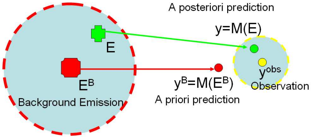
Fig. 14. A-basic methodology of top-down estimates of emissions.
