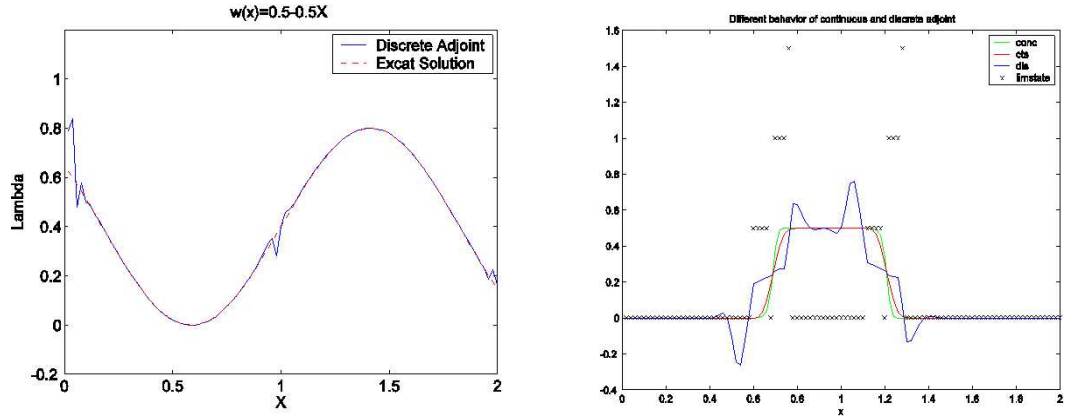
Fig. 20. (a) The discrete adjoint of a third order, upwind finite difference scheme is point-wise inconsistent with the continuous adjoint PDE near the points where the upwind direction changes (near x=1 ), and near the inflow boundaries where the numerical scheme is changed. (b) The discrete adjoints of van Leer slope limited scheme are point-wise inconsistent with the continuous adjoint PDE near the points where the limiter is active.
