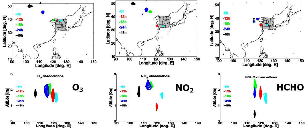
Fig. 19. Optimal location of O_3 , NO_2 , and HCHO observations to improve predictions of ground level Korean ozone (grey area). Locations of observations are shown at 6, 12, 18, 24, and 48 hours before the verification time. Note that different chemical species have to be measured at different locations according to the proposed criterion.
