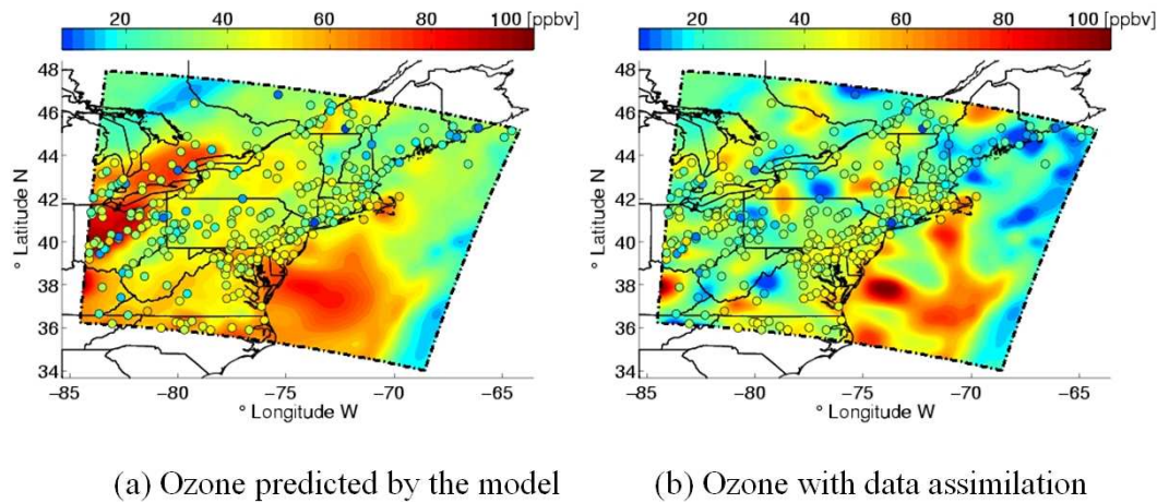
Fig. 13. Ground-level ozone at 14:00 EDT on July 20, 2004 as predicted by the model (a) without data assimilation, and (b) with data assimilation. The data is provided by the AirNow network (shown as circles colored by the measured ozone level).
