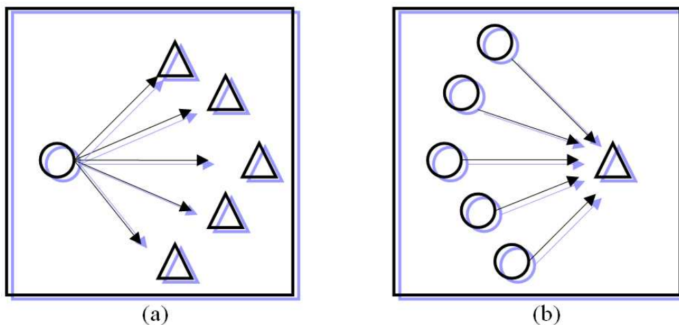
Fig. 4. (a) Direct sensitivity analysis is a source-oriented approach: the perturbation from one source is evolved and is followed by many receptors. (b) Adjoint sensitivity analysis is a receptor-oriented approach: perturbations from many sources are evolved simultaneously, and their effect is measured at one receptor.
