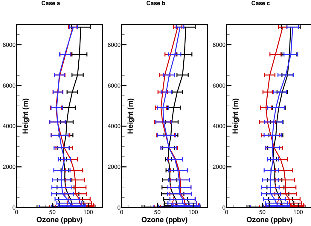
Fig. 18. Domain-averaged vertical profiles (with standard deviation) of the ozone observations (black) and the corresponding predictions before (red) and after assimilation (blue). Cases a: AirNow surface measurements; Case b: DC-8 aircraft measurement; Case c: all available measurements.
