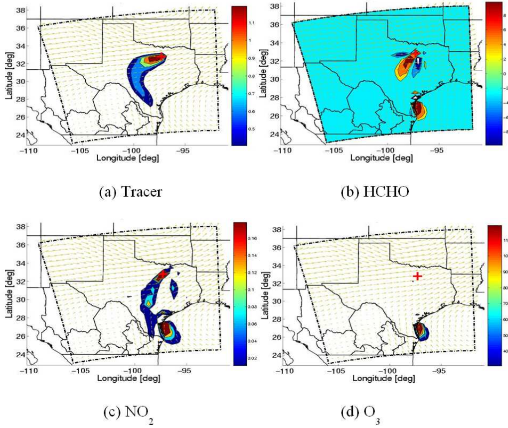
Fig. 5. (a) Tracer; (b) HCHO; (c) NO 2 ; (d) O 3 . Time-integrated areas of influence of various species on the Dallas-Fort-Worth O 3 concentration at 9pm July 2, 2004.
