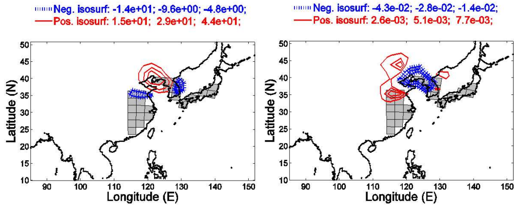
Fig. 6. The O 3 (left) and NO 2 (right) sections of the dominant model singular vectors for a 24 hour simulation of chemistry and transport over Asia. The simulated conditions correspond to March 4, 2001. The error norm at the final time is focused on the ground level O 3 and NO 2 over China, Korea, and Japan (grey area).
