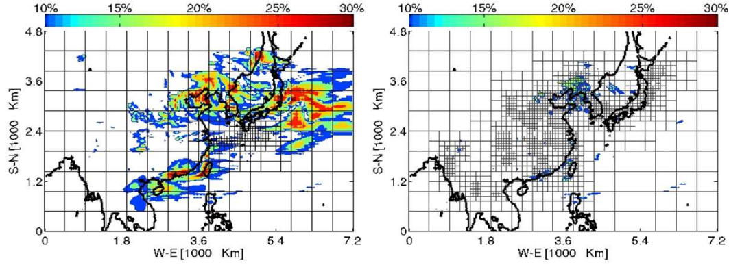
Fig. 22. The grid structure after AMR adaptation for a pollution simulation in east Asia on March 1, 2001. The horizontal grid resolution ranges between 80x80 km and 10x10 km. The grid is automatically refined in areas of higher emissions. (a) The errors in \text{NO}_2 for the coarse grid simulation. (b) The \text{NO}_2 errors on the adaptive grid.
