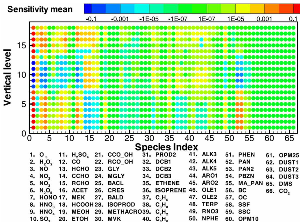
Fig. 17. Sensitivity of ozone predictions to initial conditions
