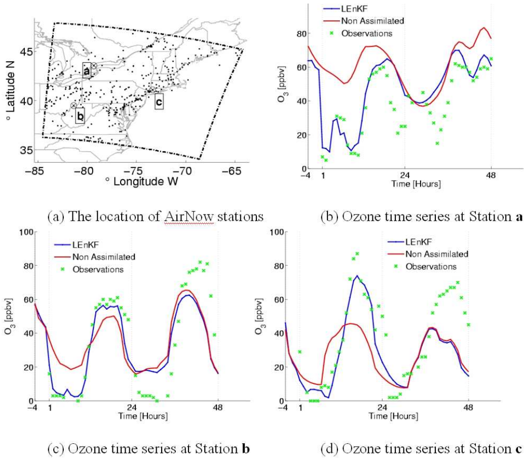
Fig. 12. The location of AirNow stations and the time evolution of ozone at three selected stations.
