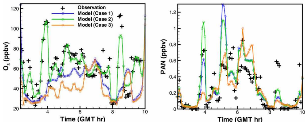
Fig. 16. Comparison of model predictions between three assimilation tests. The measurements that were assimilated: case 1, \text{NO}_y ; case 2, \text{O}_3 , \text{NO} , \text{NO}_2 , \text{HNO}_3 , PAN, and \text{RNO}_3 ; case 3, \text{NO}_y , \text{NO} , \text{NO}_2 , \text{HNO}_3 , PAN, and \text{RNO}_3 . All measurements are from the P3-B. Observation uncertainties assigned for \text{O}_3 , \text{NO} , \text{NO}_2 , \text{NO}_y , \text{HNO}_3 , PAN, and \text{RNO}_3 are 8%, 20%, 20%, 18%, 100%, 100%, and 100%, respectively.
