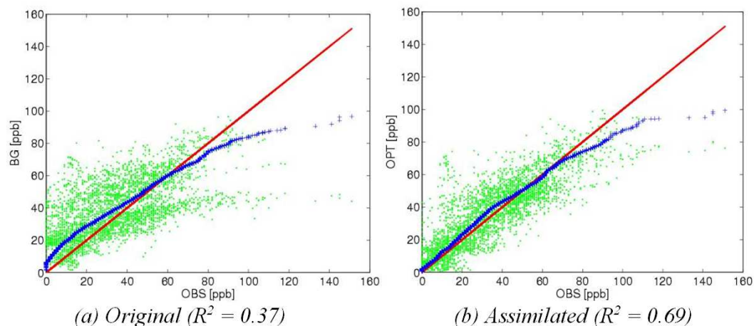
Fig. 10. Scatter- and quantile-quantile plots of model predictions versus observations (a) for the original model predictions before data assimilation, and (b) after data assimilation. The R^2 measure of model-observations agreement improves considerably.
