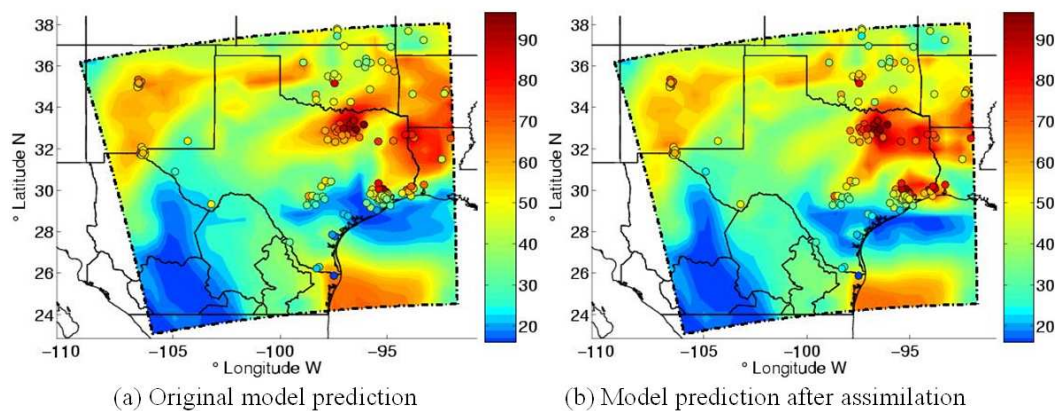
Fig. 9. (a) Original model prediction; (b) Model prediction after assimilation. Ground level ozone distribution in East Texas at 6pm CST July 16, 2004 (a) before data assimilation, and (b) after data assimilation. The colored circles represent the AirNow stations and their measured values. Data assimilation uses only AirNow ozone data and adjusts for the initial concentrations of all chemical species.
