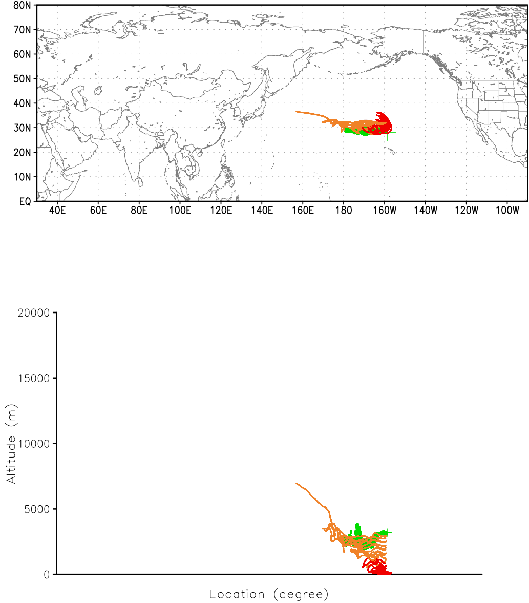
INTEX-B DC8-Low-Alt1 back traj flight 11
