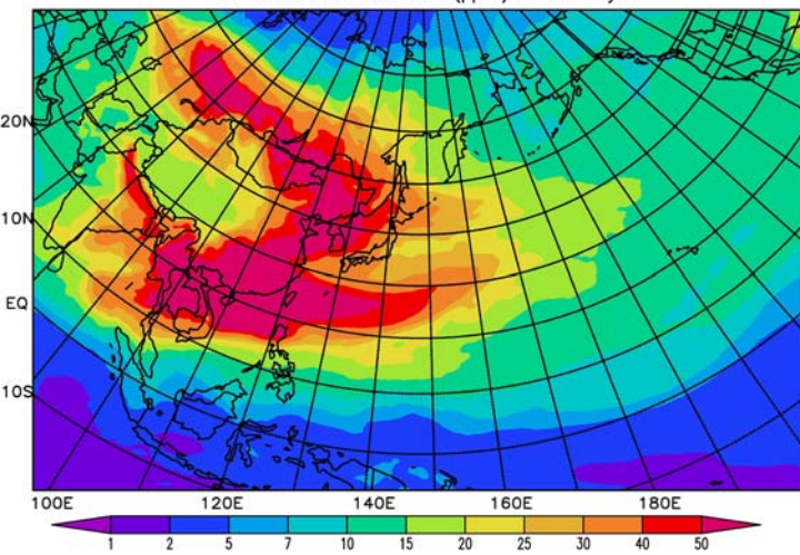
Biomass CO Concentration (ppbv) at 3km layer
