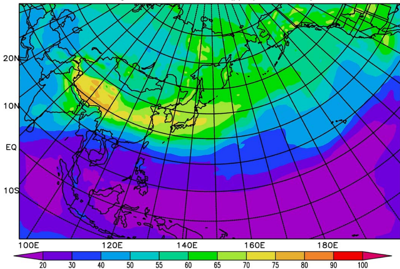
Average Ozone Concentration (ppbv) at 3 km layer
