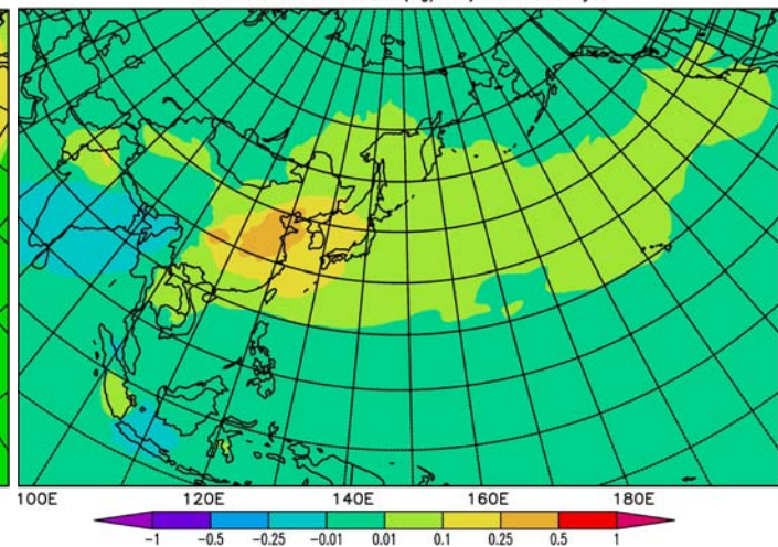
Biomass BC Concentration (ug/m3) at 3km layer
