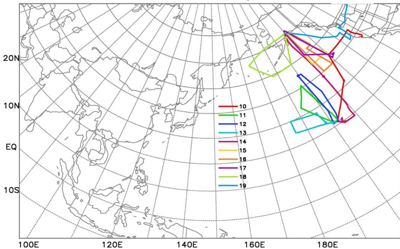
INTEXB C130 Pacific flight tracks
