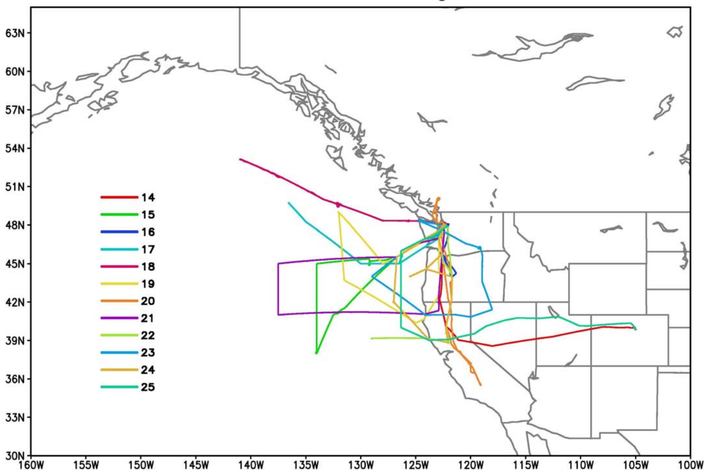
INTEXB C130 Pacific flight tracks
