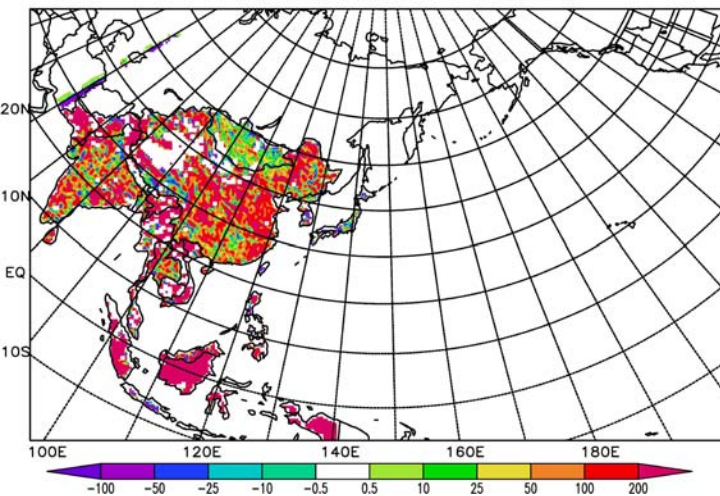
Delta CO Concentration (ppbv) at 3 km layer
