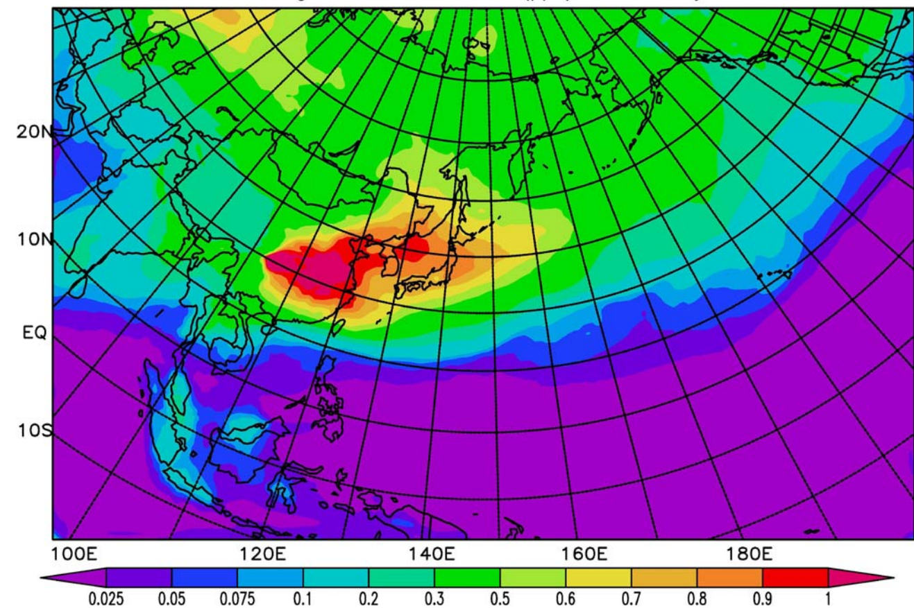
Average PAN Concentration (ppb) at 3 km layer
