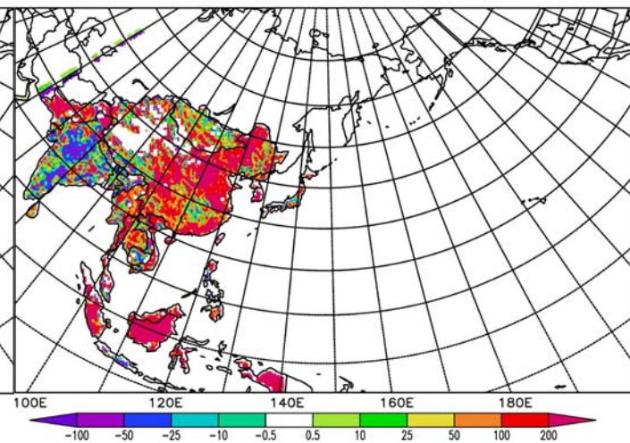
Delta BC Concentration (ug/m3) at 3 km layer
